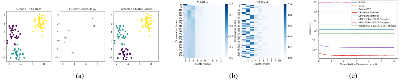
Figure 5: (a) One random sample from a mixture of 3 Gaussians (left). Centroids learned by R-CRP (center). Predicted class labels by R-CRP (up to an arbitrary aliasing) (right). (b) Evolution of cluster assignment priors p(z_t | o_{<t}) (left) and cluster assignment posteriors p(z_t | o_{\leq t}) (right) as more data are observed from the Mixture of Gaussians. (c) R-CRP is slower than most online baselines but significantly faster than offline baselines.
