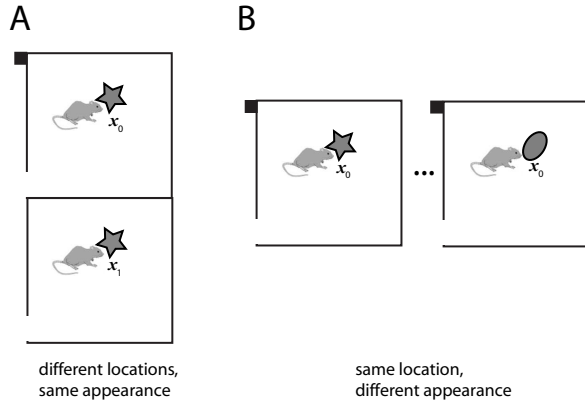
Figure 7: Uses of the grid-cell code: non-metric place-label readout. The black square represents home-base or the rat's starting location. A Metrically updated place-labels that themselves convey no metric information can help to differentiate separate but similar looking locations ( x_0 versus x_1 ). B A landmark may change appearance over time; however, the metric updating of dMEC phases as the rat moves from a reference point to the landmark generates an invariant dMEC phase vector at the landmark. The consistent dMEC state helps to correctly identify a location despite the inconsistency of sensory cues.
