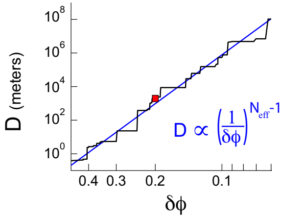
Figure 3: Capacity grows as a power of the phase resolution within lattices. The maximum uniquely representable distance grows as a power of the phase resolution, D \propto (1/\delta\phi)^{N_{\text{eff}}-1} . Red dot: phase uncertainty of \delta\phi = 1/5 . ( N = 12 , with first lattice period = 30 cm, and increments of 4 cm per subsequent lattice.) The fit parameter N_{\text{eff}} \simeq 10.7 , smaller than N = 12 , but of similar magnitude.
