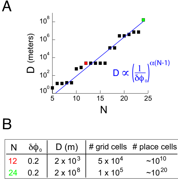
Figure 4: Capacity grows exponentially with the number of lattices. A The maximum uniquely representable distance, D , grows exponentially with the number of lattices, D \propto (1/\delta\phi_0)^{\alpha(N-1)} . For all lattices, the phase resolution is \delta\phi_0 = 1/5 ; as in Figure 3, the first lattice period is 30 cm, with 4 cm increments per subsequent lattice. The fit parameter is \alpha \simeq 0.62 . Red dot: N = 12 . Green dot: N = 24 . B 12 lattices with uniformly spaced periods from 30 cm to 74 cm with \delta\phi = 0.2 can unambiguously represent a \sim 2 \text{ km} \times 2 \text{ km} area with 6 cm \times 6 cm resolution. If 5000 neurons build each lattice, that would require \sim 5 \times 10^4 neurons. To cover the area with sparse unimodal place-cell like encoding (with 10 neurons per (6 \text{ cm})^2 block) would require \sim 10^{10} neurons, compared to the estimated 10^5 neurons in rat dMEC (Amaral et al., 1990; Mulders et al., 1997), which could unimodally represent at most \sim 6 \text{ m} \times 6 \text{ m} with (6 \text{ cm})^2 resolution. With 24 lattices, D \sim 2 \times 10^8 \text{ m} (with 6 cm resolution) in each direction, hugely in excess of the representational requirements of rats.
