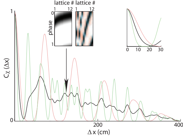
Figure 6: Decorrelation of dMEC population response with distance. Black line: Cross-correlation between the full dMEC vectors (representing activity in all phases, all lattices) corresponding to pairs of locations separated by distance \Delta x . Green (Pink) curves: Cross-correlations for the dMEC phase vector of only the two smallest (largest) lattices. The dMEC population correlation is high and monotonically decreasing with \Delta x for small separations (central peak, magnified in rightmost inset ): in this regime, distances in the space of dMEC responses are proportional to distances in real space. However, the dMEC population vector has completely decorrelated for \Delta x comparable to the width of a blob in the largest lattice (full-width at half-maximum (FWHM) of \sim 18 cm; the central peak width in the green (pink) curve is approximately the blob width in the smallest (largest) lattice), beyond which dMEC correlations begin to vary non-monotonically. Central insets: Two sample dMEC population vectors, representing two positions separated by \Delta x = 140 cm, to illustrate the degree of decorrelation in the population activity. Abscissa: index of different lattices, arranged in order of increasing period. Ordinate: phase of the active population within the corresponding lattice. Grayscale intensity represents the analog level of activity (black=maximally active). Center left: the population vector at x = 80 cm; center right: the population vector at x = 220 cm. Parameters: N = 12 1-d lattices, periods uniformly spaced in [30, 74] cm. The binary population vector \chi ( N \times M dimensions) has \chi(\alpha, i) = 1 if i = \text{ceil}[M(x \bmod \lambda_\alpha)/\lambda_\alpha] , and zero otherwise. M = 100 is the number of different phase bins per lattice. The population activity vector \vec{r} = \{r_{\alpha,i}\} is the convolution within each lattice of the phase vector with a hanning kernel, so that although the activity of the \alpha, i th phase group peaks at \phi_{\alpha,i} , it also responds to neighboring phases, with FWHM of 1/4 of the total lattice period.
