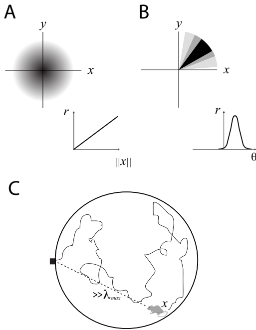
Figure 8: Uses of the grid-cell code: explicit metric readout. A An example of an explicit metric readout of the dMEC phase code: if the firing rate of a readout cell is proportional to displacements of the rat from a starting location, small changes in the neural response correspond to small changes in rat location and vice versa, and constituting an explicitly metric code for displacement. Top: 2-d; bottom: 1-d. B An example metric readout for angular displacements: The firing of a cell is proportional to closeness to a reference orientation. Top: 2-d; bottom: 1-d. C Explicitly metric readouts may be used to compute the straight-line path home after random excursions over long distances. The black square represents home-base.
